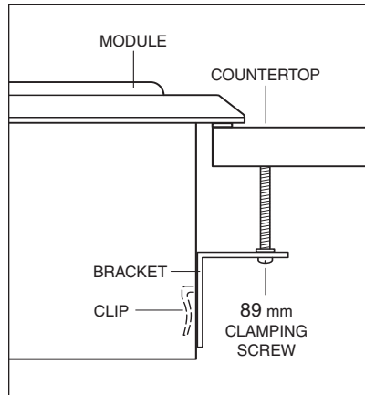
Installation brackets
